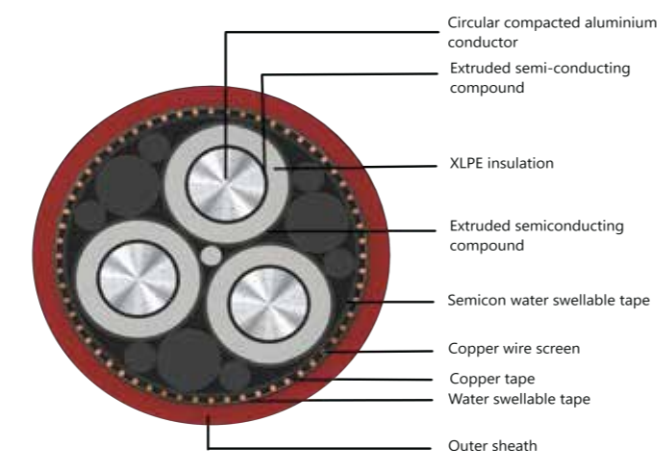
POLYCAB MV AL BS 7870-4-20 6.35/11 KV - Medium Voltage Copper wire screened Cable, 6.35/11 (12) KV AC
